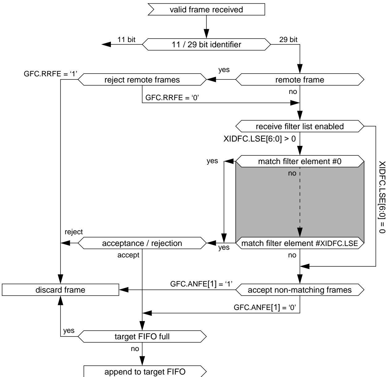
Figure 6 Extended Message ID Filter Path
