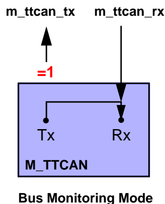
Figure 3 Pin Control in Bus Monitoring Mode
