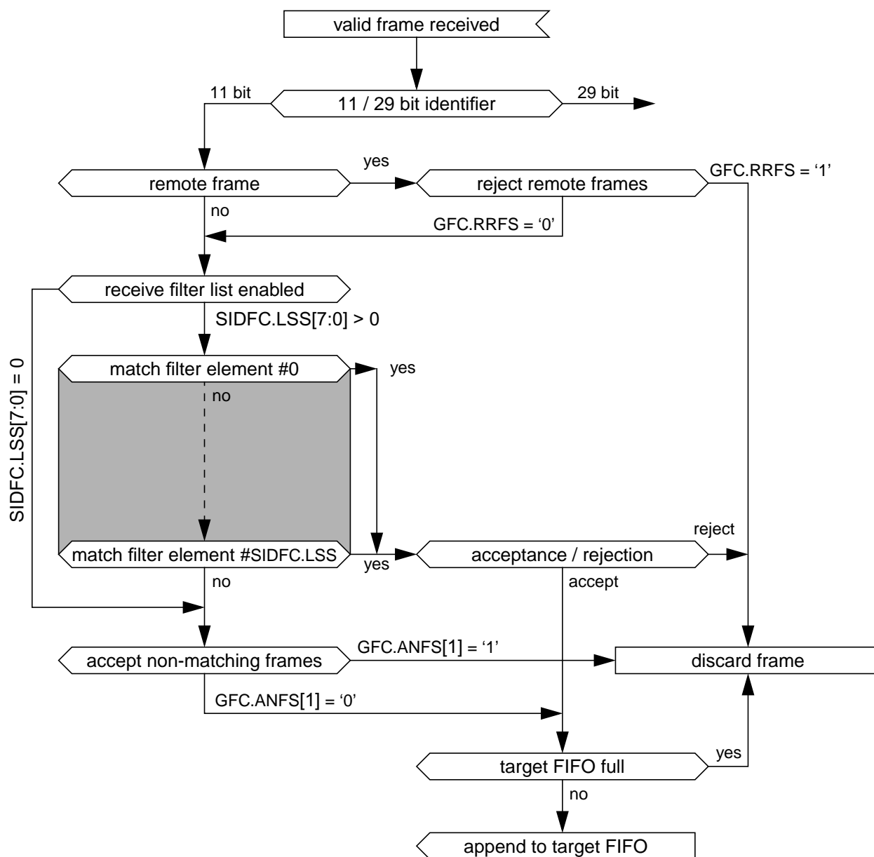
Figure 5 Standard Message ID Filter Path
