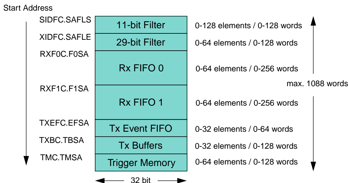
Figure 2 Message RAM Configuration
