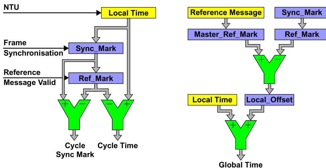
Figure 9 Cycle Time and Global Time Synchronization
