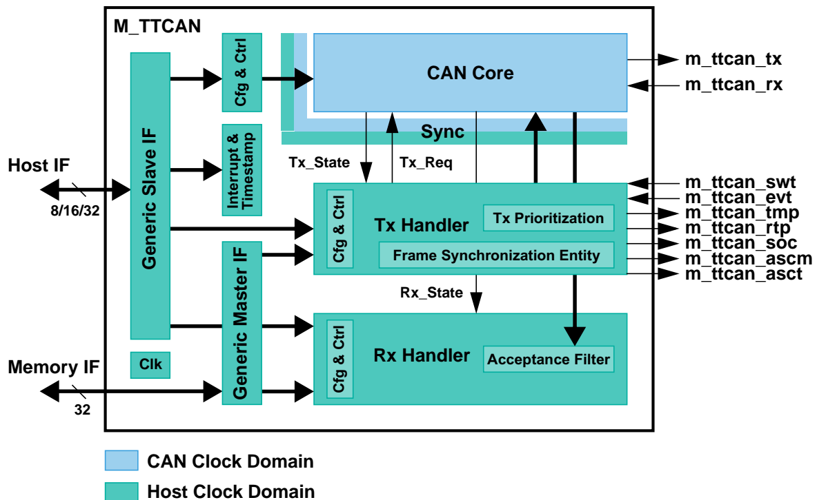
Figure 1 M_TTCAN Block Diagram
