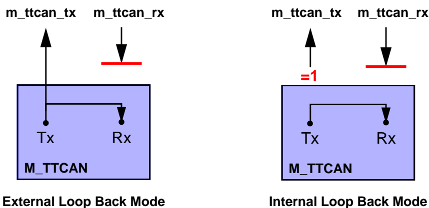
Figure 4 Pin Control in Loop Back Modes
