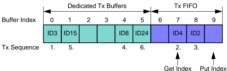
Figure 7 Example of mixed Configuration Dedicated Tx Buffers / Tx FIFO
